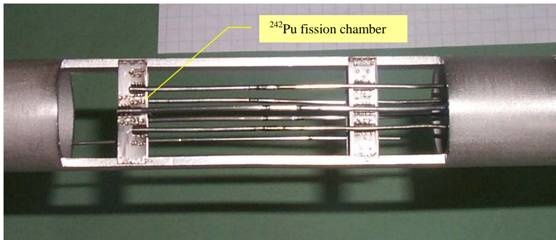
Detail of the experimental rig with the ^{242}\text{Pu} fission chamber together with other subminiature fission chambers.
