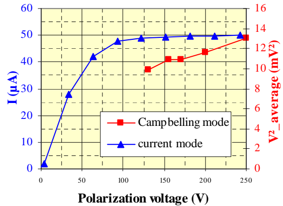
The experimental data of the Pu-242 fission chamber: linearity of the response and polarization voltage dependence of the signals in current and Campbelling mode.
