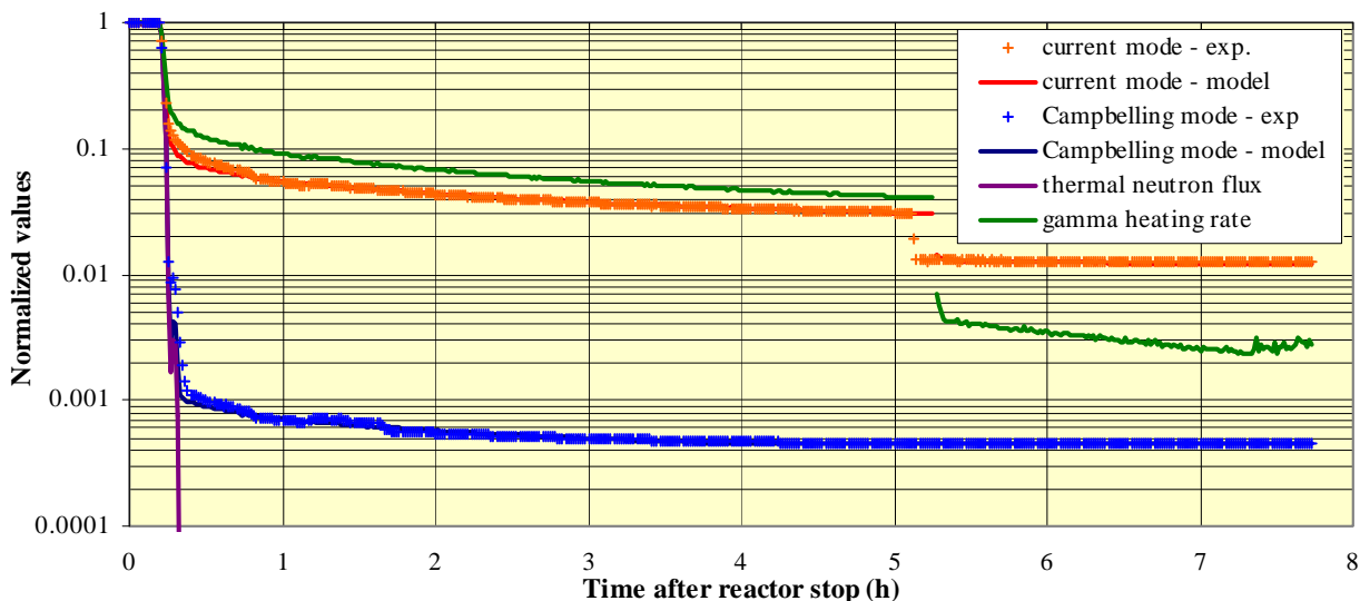
Normalized Pu-242 fission chamber data just after the reactor stop: signals in current and Campbelling mode together with the fitted curves. After five hours the experimental rigs were unloaded from the reactor. The recorded thermal neutron flux and gamma heating rate data are also shown.
